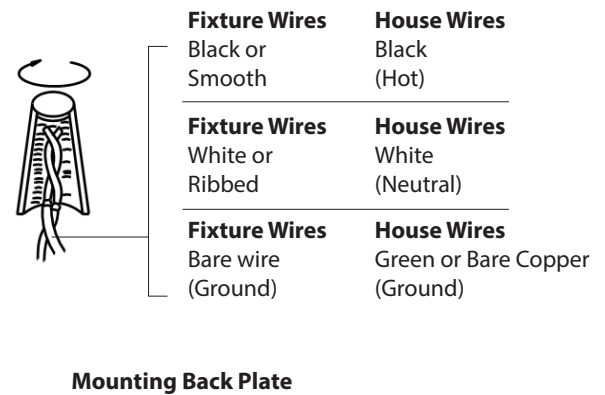
Fig.2 Wiring
