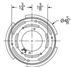
Mounting Backplate Dimensions
