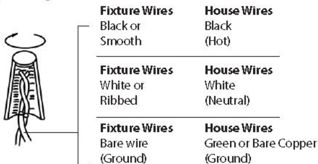
Fig.2 Wiring
