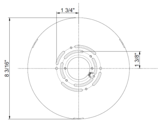
MOUNTING BACK PLATE
