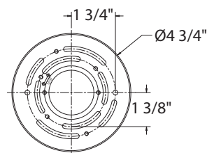
Mounting Back Plate Dimensions
