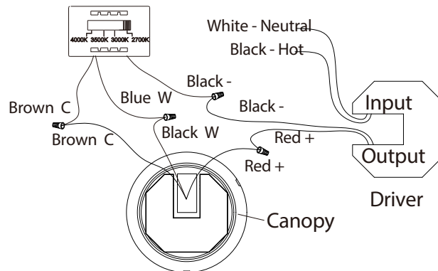
Fig.3 Driver Wires
