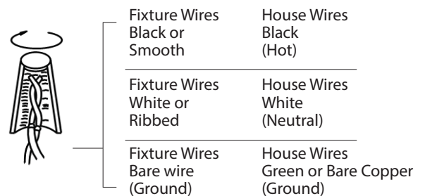
Fig.2 Wiring
