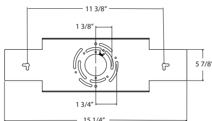
Fig.4 Mounting Plate Dimensions
