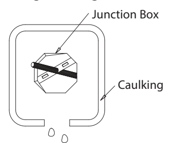
Fig. 4 Sealing
